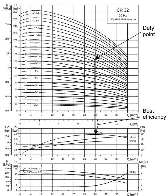
Fig. 10 Example of a CR pump's duty point
