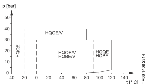
Fig. 7 Operating range of standard shaft seals for CR, CRI, CRN 1s-155
