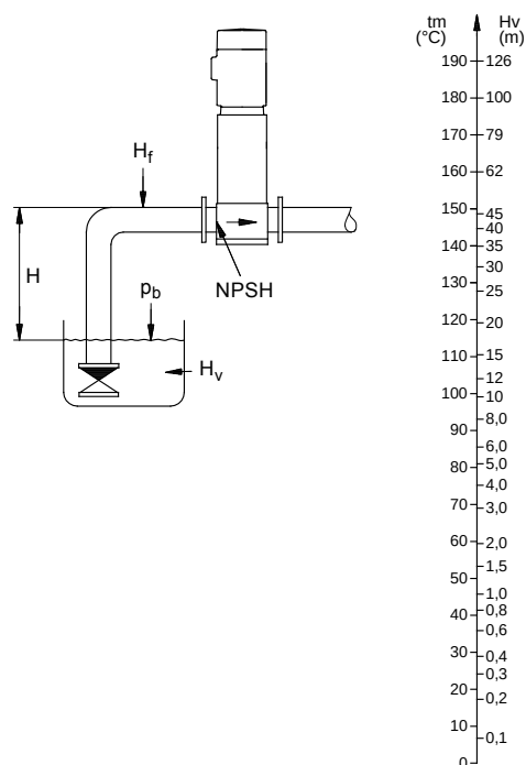
Fig. 18 Minimum inlet pressure, NPSH
